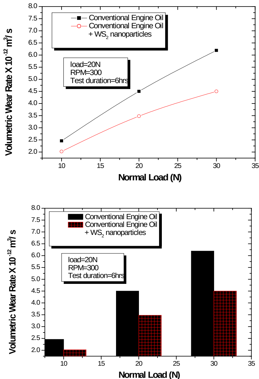
Figure 3 Variation of volumetric wear rate with normal load of 20 N at 300 rpm.
