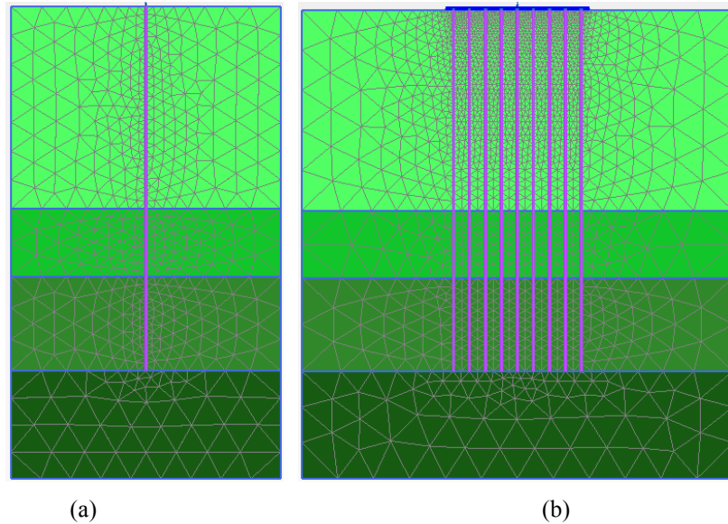
Figure 8 Mesh generation of pile group having coarseness of medium mesh; (a) single pile row and (b) 9×1.
