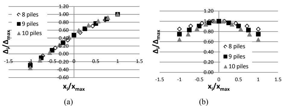
Figure 20 Influence of number of piles to the normalized settlement profile; (a) combined axial load and moment case and (b) axial load case.
